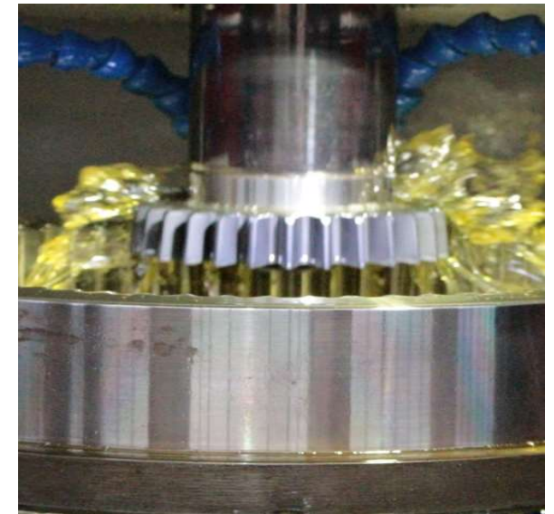
CNC shaping machines (3 sets) CNC (3台)
